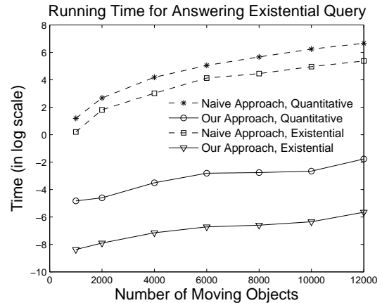
Figure 12: Existential queries.
