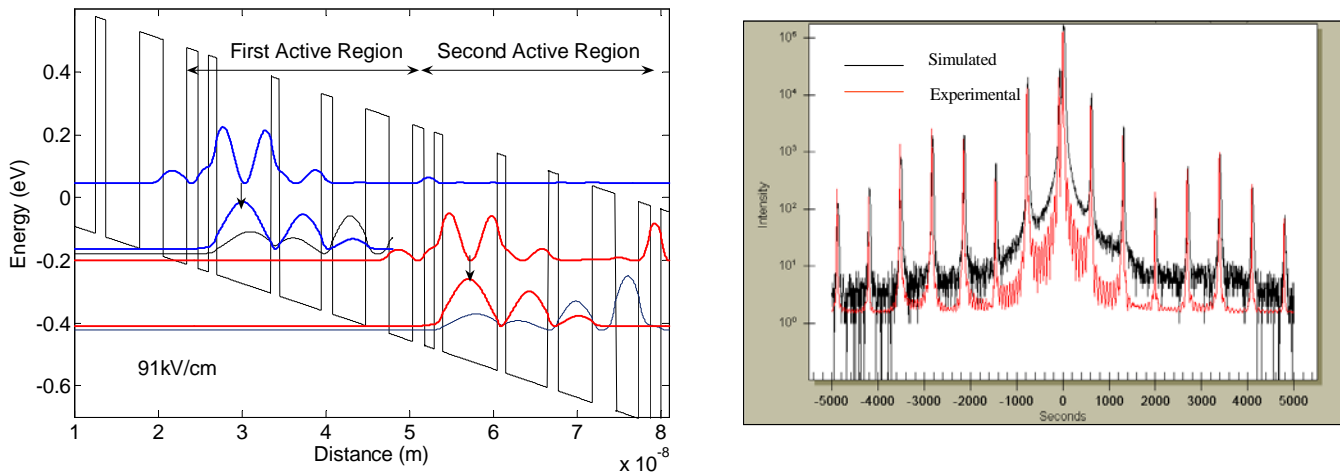
Figure 2 – (a) Band diagram for injectorless QCL at applied voltage of 91kV/cm showing the transition (b) Experimental and simulated x-ray diffraction curve of a strain-balanced injectorless QC-laser
