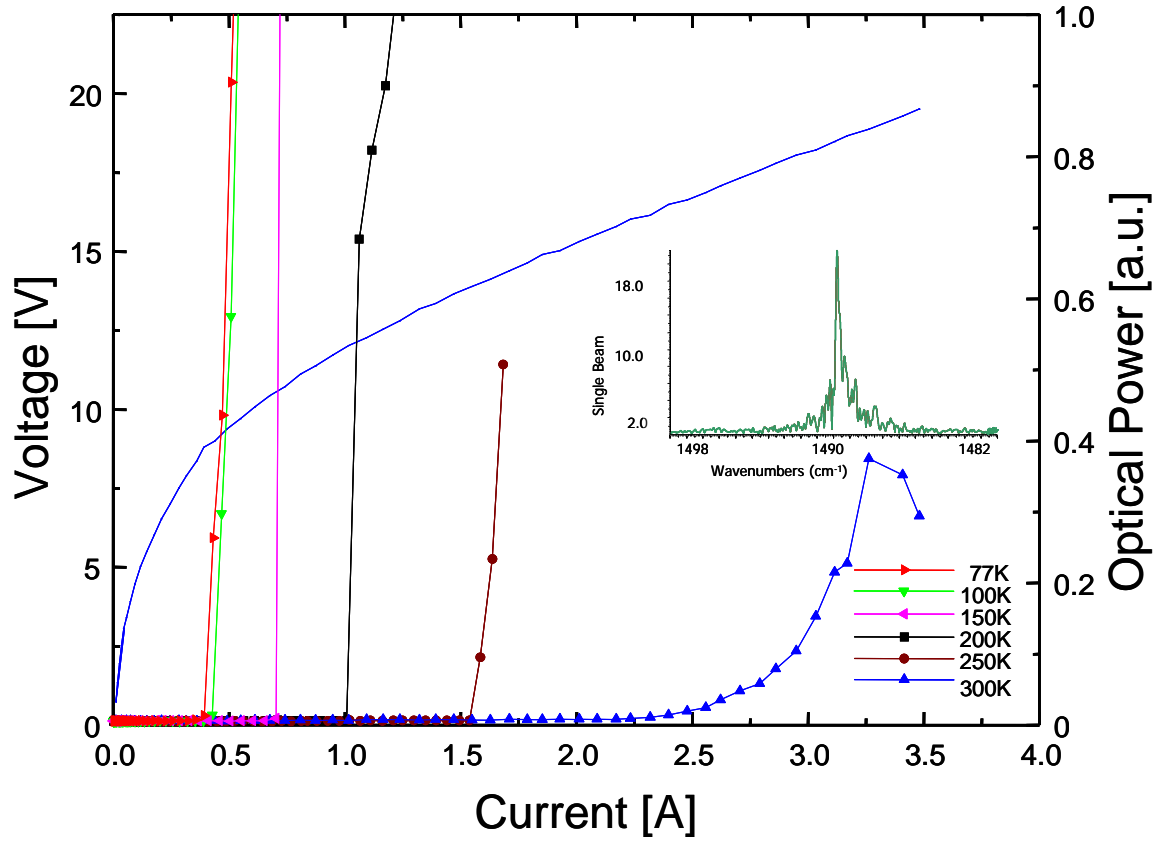
Figure 1 – (a) Light-current-voltage (L-I-V) measurement for a 2.1mm long and 25µm wide laser chip at different heat-sink temperatures with inserted picture shows the light output@ 6.7µm
