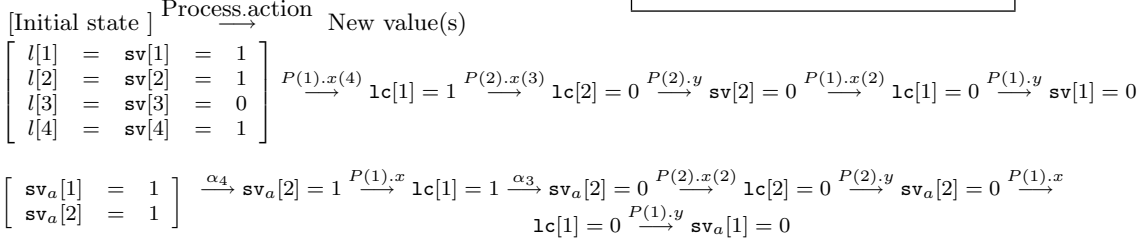
Figure 2: This is an example of the application of the transformation. Upper left figure shows the actions of \mathcal{Q}(N) . Upper right figure shows the actions of \mathcal{Q}_a(N) . For simplicity the part of each action specifying the variables left unchanged is not shown. For P(id, N) actions x are transformed by rule T2, actions y by rule T3, and actions \alpha_i are added because of rule T0. The upper sequence is a behavior segment of the original system. The bottom sequence is the corresponding behavior segment of the abstract system. The projections of two behavior segments over the variables in V_{nsv} \cup \{sv[1]\} are stuttering equivalent. Only the relevant values are displayed in the figure.
