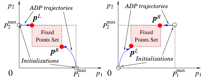
Fig. 2. Examples of the trajectories of the power profiles under the ADP algorithm for a two-user network with Type I (left) or Type II (right) utility functions. In both cases, from the indicated initializations the power profiles will monotonically converge to the indicated "corner" fixed points.
