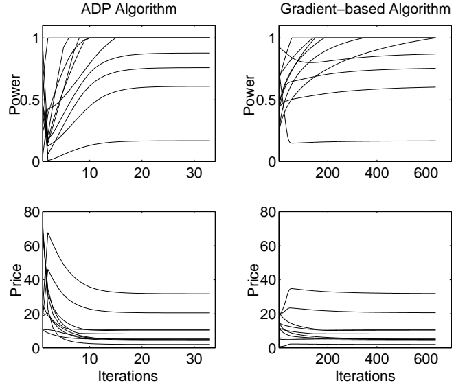
Fig. 3. Convergence of the prices and powers for the ADP algorithm (left) and a gradient algorithm (right) in a network with 10 users and logarithmic utility functions. Each curve corresponds to the power or price for one user with a random initialization.
