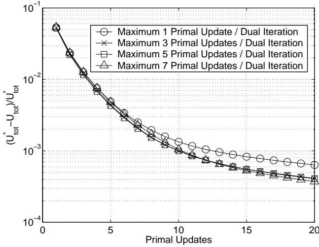
Fig. 5. Number of Primal Updates needed for the DADP convergece
