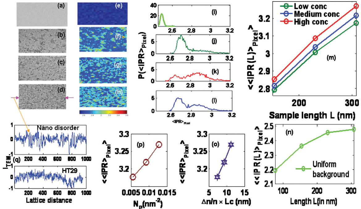
FIG. 2. (Color) [(a)–(d)] Representative grayscale images of uniform background of dielectric thin film and dielectric nanoparticles on dielectric thin films with increasing particle concentration (or disorder strength). [(e)–(h)] Corresponding IPR images. [(i)–(l)] Distribution P(\langle \text{IPR} \rangle_{\text{Pixel}}) plots. (m) \langle \text{IPR}(L) \rangle_{\text{Pixel}} vs L plots for three different disordered samples, and (n) Same as (m) for uniform sample. (o) \langle \langle \text{IPR}(\Delta n/n_0 \times L_c) \rangle \rangle vs (\Delta n/n_0 \times L_c) plot and (p) \langle \langle \text{IPR}(N_p) \rangle \rangle vs N_p plot. (q) I_{\text{TEM}}(L) plots for nanodisordered sample (top) and the same for a HT29 cell [Fig. 3(a)] (bottom).
