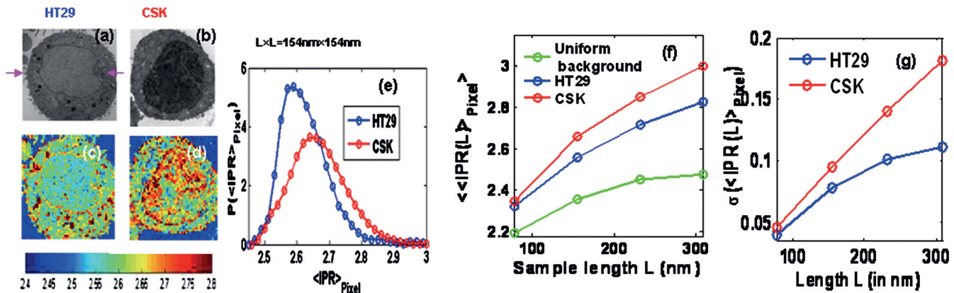
FIG. 3. (Color) [(a) and (b)] Representative TEM images of HT29 cells and CSK cells. [(c) and (d)] Corresponding \langle IPR \rangle_{\text{Pixel}} image. (e) Relative \langle IPR(L) \rangle_{\text{Pixel}} distributions for HT29 and CSK cells. (f) Ensemble averaged \langle \langle IPR(L) \rangle_{\text{Pixel}} \rangle vs L plots for (i) uniform sample (or background), (ii) HT29 cells, and (iii) CSK cells. (g) Standard deviation \sigma(\langle IPR(L) \rangle_{\text{Pixel}}) vs L plots for HT29 cells and CSK cells. Because of the large number of samples ( \sim 50\,000 ), the error bars are negligible.
