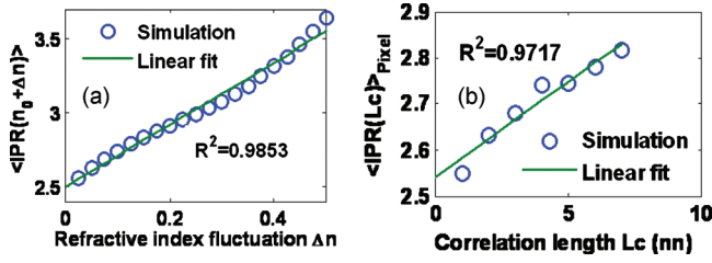
FIG. 1. (Color) Numerical simulation results: (a) \langle \text{IPR}(\Delta n) \rangle vs \Delta n and (b) \langle \text{IPR}(L_c) \rangle vs L_c plots.
