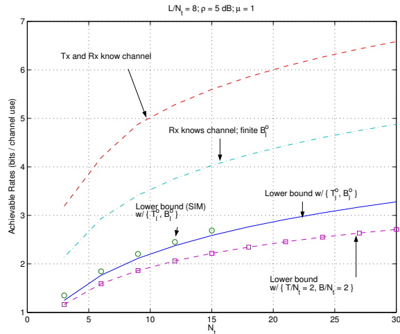
Fig. 3. Achievable rate versus number of transmit antennas N_t with different assumptions about channel knowledge at the receiver and transmitter.
