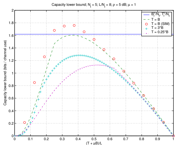
Fig. 4. Lower bound on capacity versus normalized training and feedback (T + \mu\bar{B})/L .
