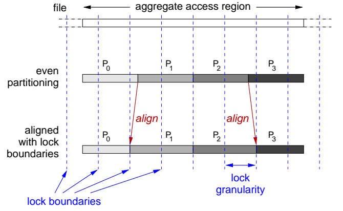
Fig. 2. File domains produced by the even and lock-boundary aligned partitioning methods.
