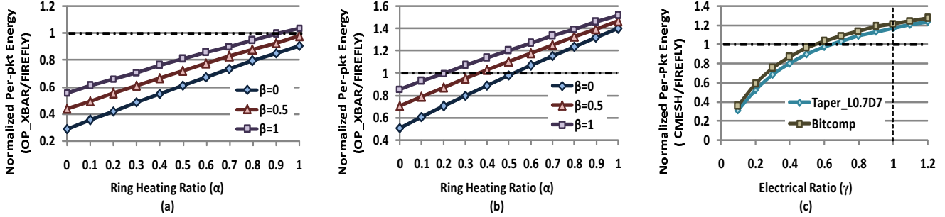
Figure 15: Technology sensitivity comparing OP_XBAR vs. Firefly under (a) bitcomp and (b) taper_L0.7D7 traffic and (c) CMESH vs. Firefly under taper_L0.7D7 and bitcomp
